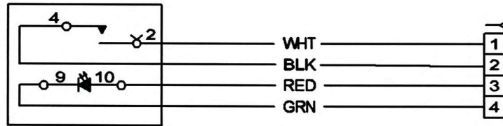
WIRING DIAGRAM
